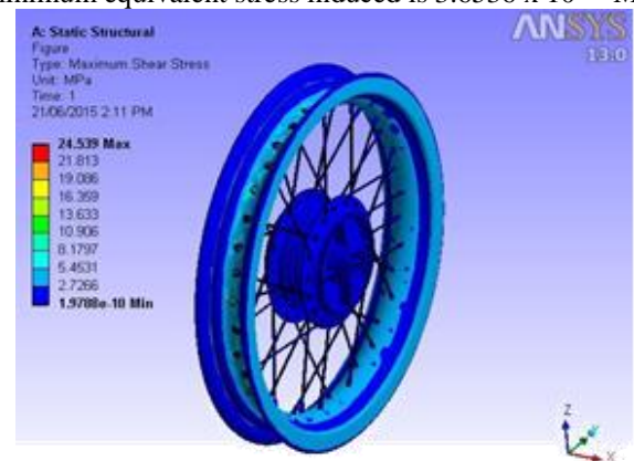
Fig. 12. Maximum Shear Stress
