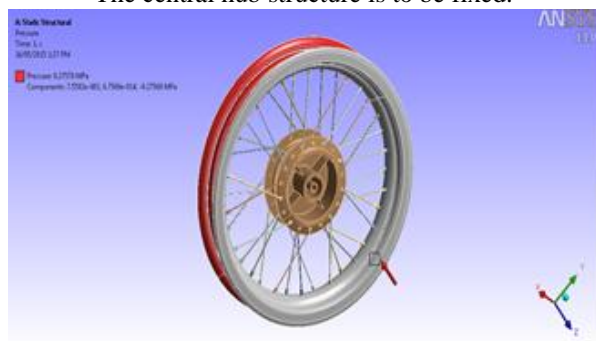
Fig. 10. Pressure
