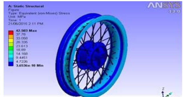
Fig. 11. Equivalent (Von- Mises) Stress
