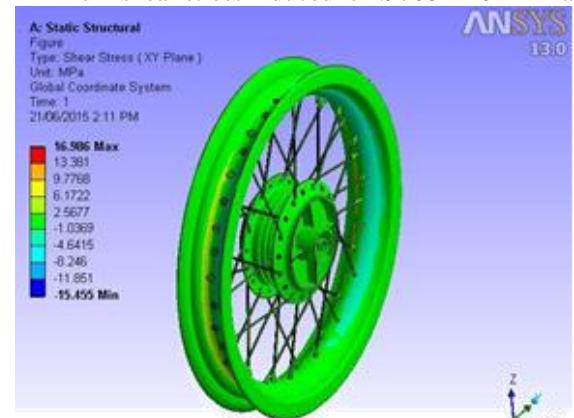
Fig. 13. Shear Stress
