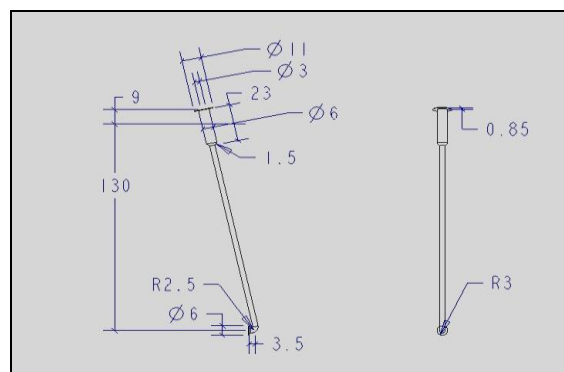
Fig.3.Geometric model of Spoke.
