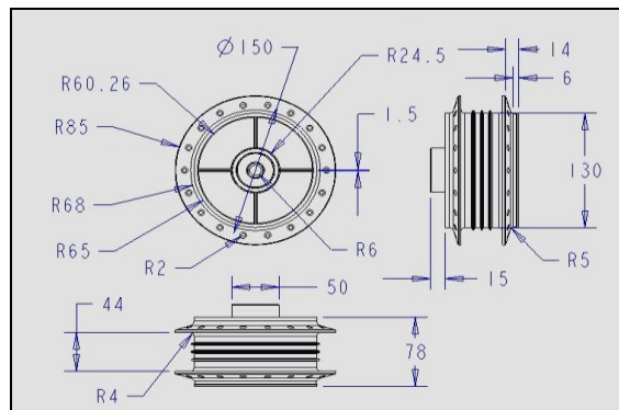
Fig.2.Geometric model of Hub.
