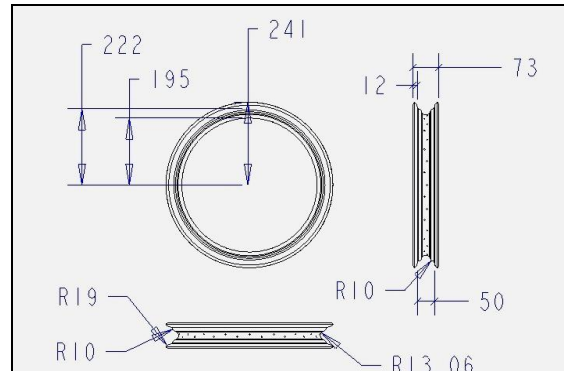
Fig.1.Geometric model of existing rim.
