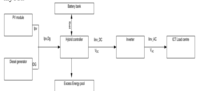
Figure 3: configuration of PV/Diesel Hybrid Power Supply
