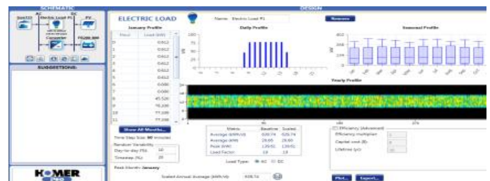
Figure 4: Homer interface [7]
