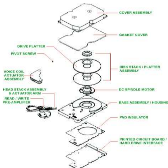
Figure 5: HDD Parts
