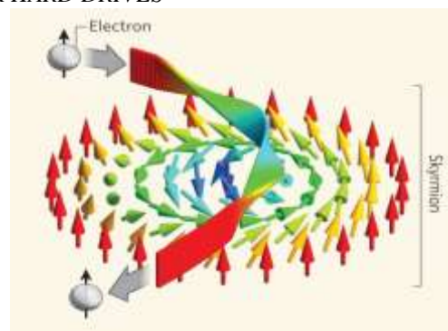
Figure 15: SKYRMIONS
