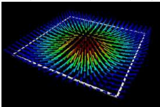
Figure 15: SKYRMIONS
