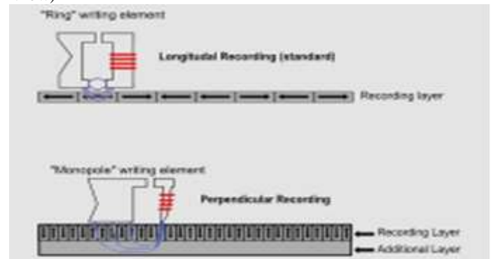
Figure 4: Longitudinal recording (standard) & perpendicular recording diagram Parts of the Hard Disk Drive
