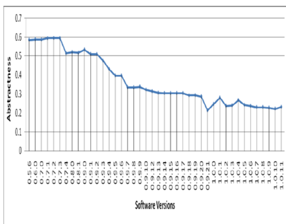
Fig. 7: Average Abstraction Level of Packages.
