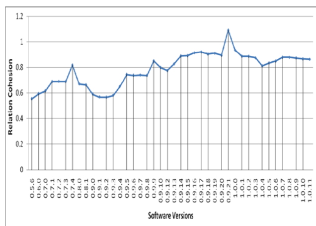
Fig. 5: Relation Cohesion Metric Trend
