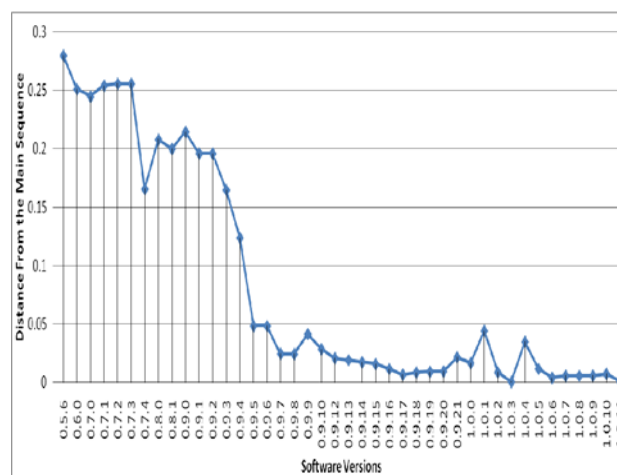
Fig.8: Distance from the Main Sequence Metric Trend
