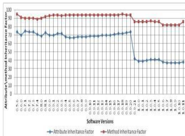
Fig.3: Attribute Inheritance Factor and Method Inheritance Factor Metrics Trends
