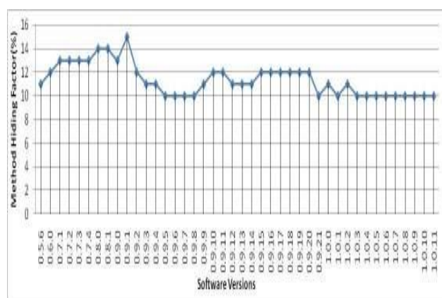
Fig.1: Method Hiding Factor (MHF) Metric Trend
