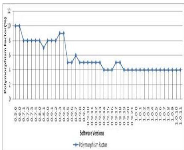
Fig. 4: Polymorphism Factor (PF) Metric Trend
