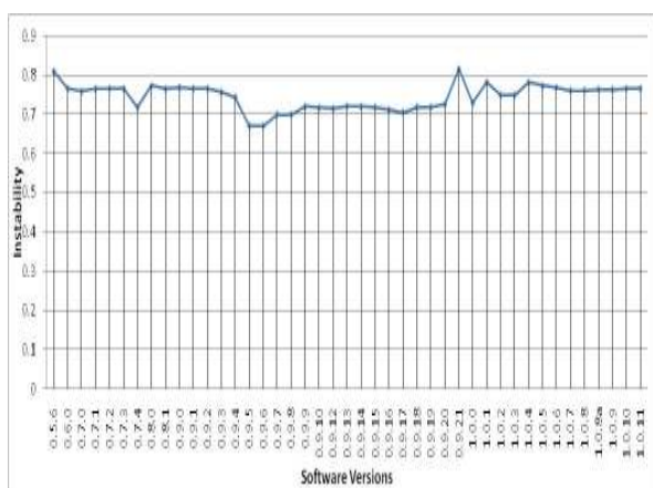
Fig. 6: Instability Metric Trend
