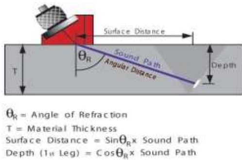
Fig-1 Ultra Sonic Testing
