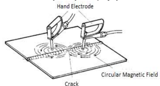
Fig-3 Magnetization using hand held electrodes
