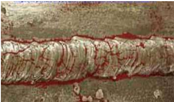
Fig-5 Indication of crack in weldments
