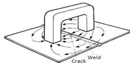
Fig-4 Magnetization using a permanent magnet
