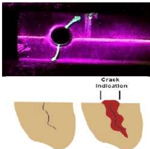
Fig-6 Liquid Penetrant Inspection of a Material
