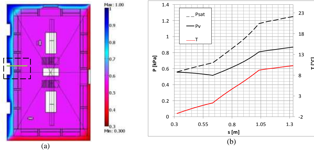
Fig. 9. Relative humidity distribution on the horizontal plane (a) with an indication of the chosen plane for the trends of vapour partial pressure ( P_v ), saturation pressure ( PSAT ) and air temperature, shown in the graph to the right (b)
