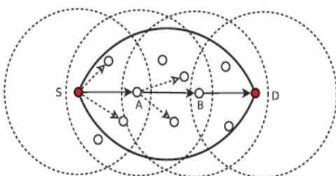
Fig2: Duplicate Relaying Is Limited in the Region Enclosed By the Bold Curve
