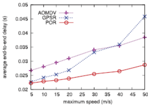
(b) Average end-to-end delay.
