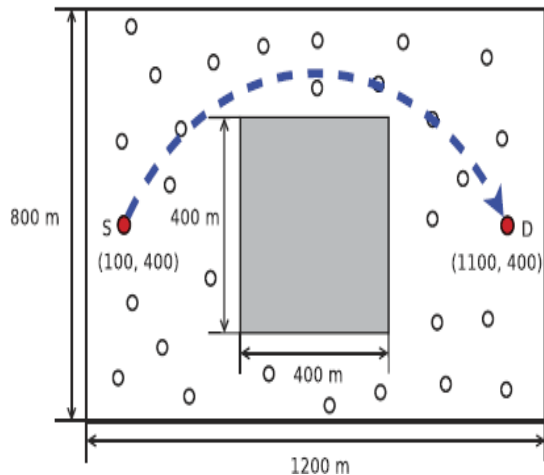
Fig5: network topology
