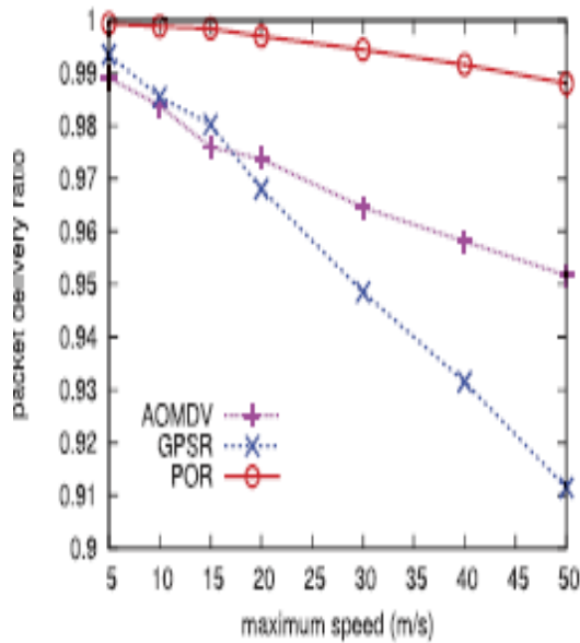
(a) Packet delivery ratio.
