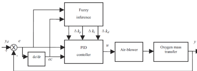
Fig.5. Block diagram of the adaptive fuzzy PID controller of DO [24]
