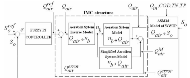
Fig.7. Nonlinear fuzzy control system [25]
