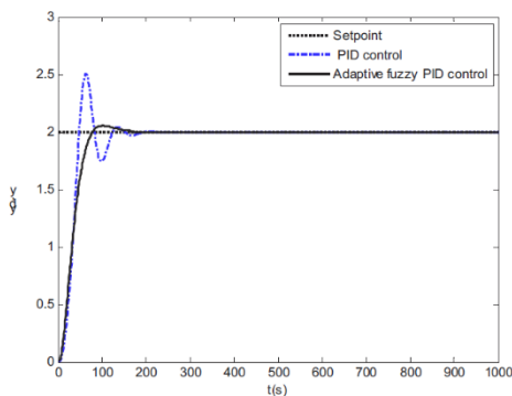
Fig.6. Results of the PID control and adaptive fuzzy PID control [24]
