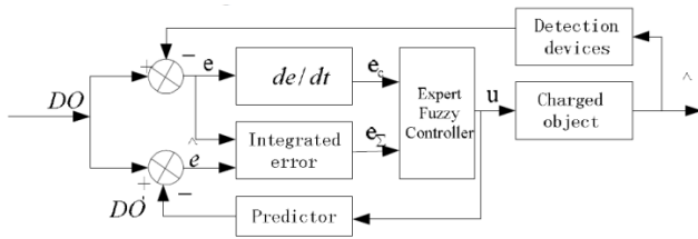
Fig.8. Predictive control based on experts fuzzy control system [28]
