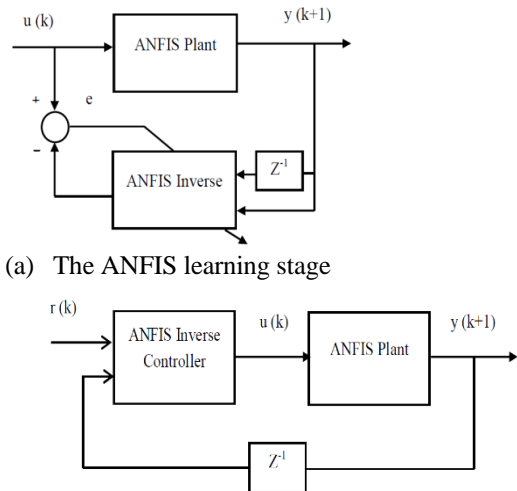
Fig. 4 The schematic diagram of inverse learning training for ANFIS [20]
