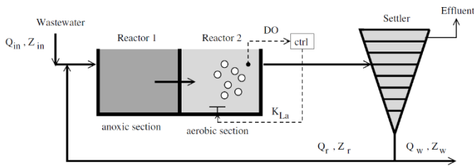
Fig. 2. General overview of simulation model [16]
