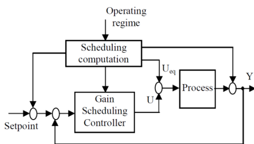
Fig. 3. Control scheme with Gain Scheduling controller type [17]
