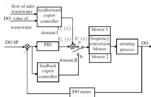
Fig.1 The schematic diagram of control system [4]
