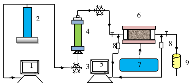
1. Pressure & Flow Control System; 2. RUSKA Pump; 3. 6-Way Valve; 4. High Pressure Vessel; 5. Pressure Acquisition System; 6. Core Holder; 7. Confining Pressure Pump; 8. Pressure Sensor; 9. Flow meter
