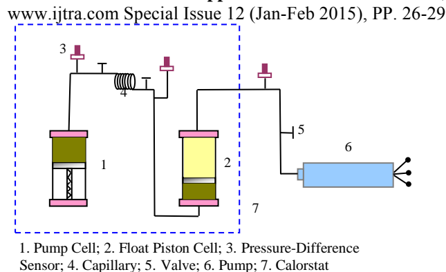
Fig.3. Schematic of RUSKA online high-pressure caplastometer.
