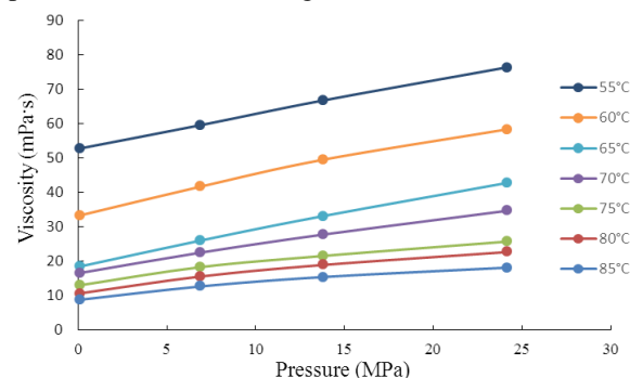
Fig.4. Viscosity sensitivity behaviors of heavy oil.
