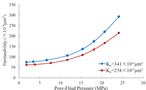
Fig.2. Permeability sensitivity behaviors of different cores.
