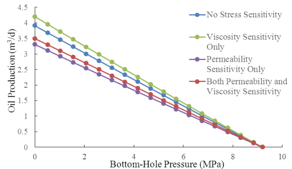
Fig.5. Oil production curves under different stress sensitivity conditions
