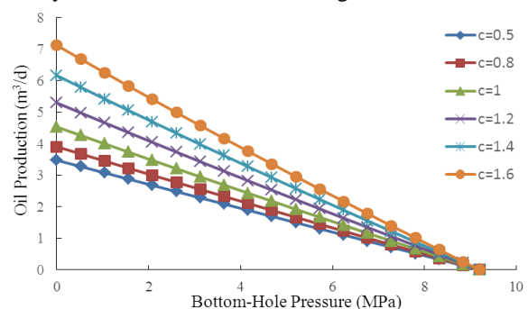
Fig.6. Productivity contrasts under different viscosity sensitivity coefficients
