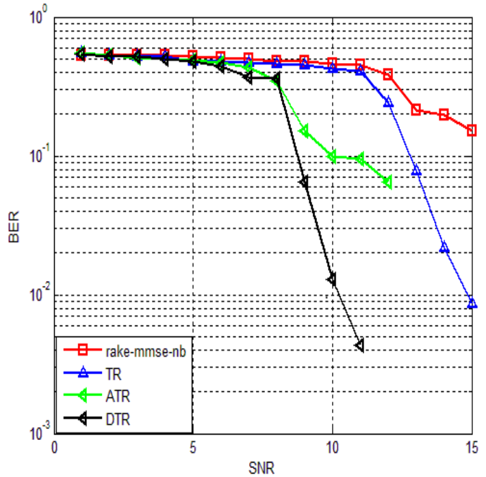
Fig3.BER performance of various non coherent UWB receivers in CM4
