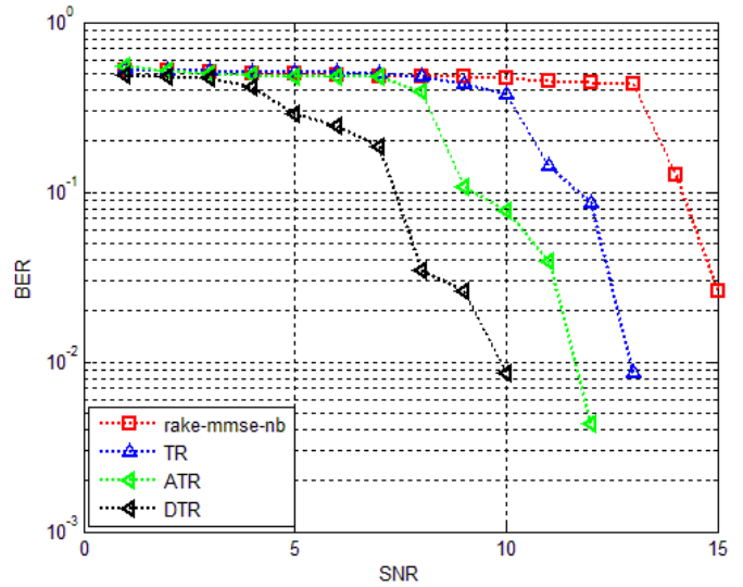
Fig2.BER performance of various non coherent UWB receivers in CM3
