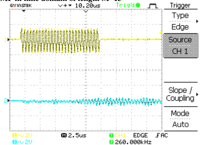
Fig.12: the input and output of the DMF for pulse modulation signal
