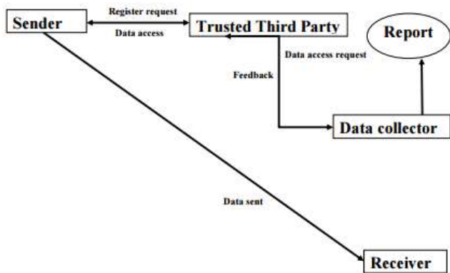
Fig. 1. Privacy-Preserving System
