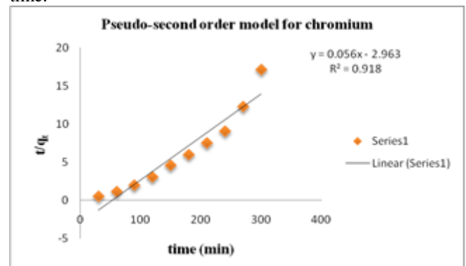
Fig 15: Pseudo second-order model for adsorption of chromium by activated Na-bentonite
