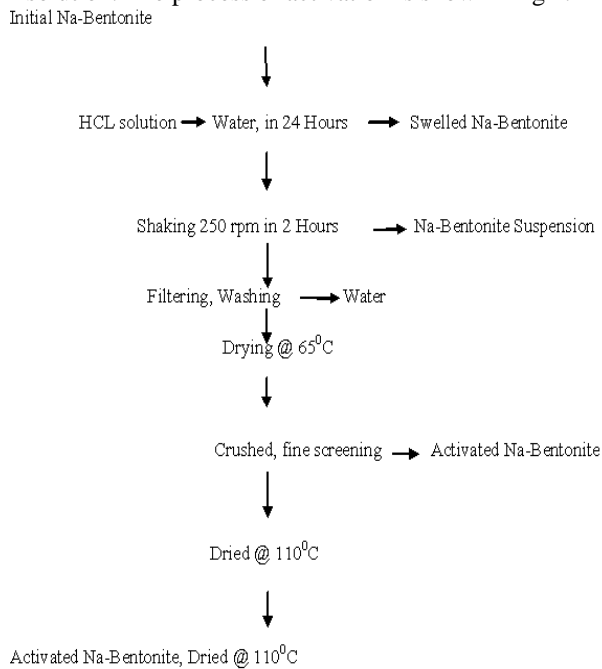
Fig 2: Activation of Sodium-bentonite
