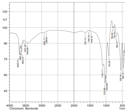
Fig 8: Interferogram for after chromium adsorption on activated Na- bentonite
