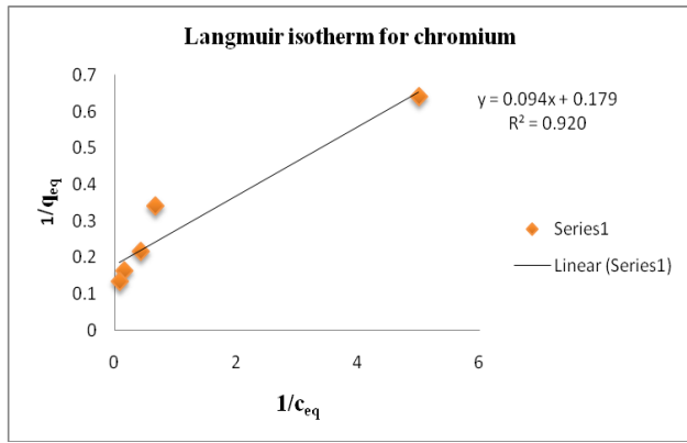
Fig 12: Langmuir isotherm plots for Chromium adsorption by activated Na-bentonite
