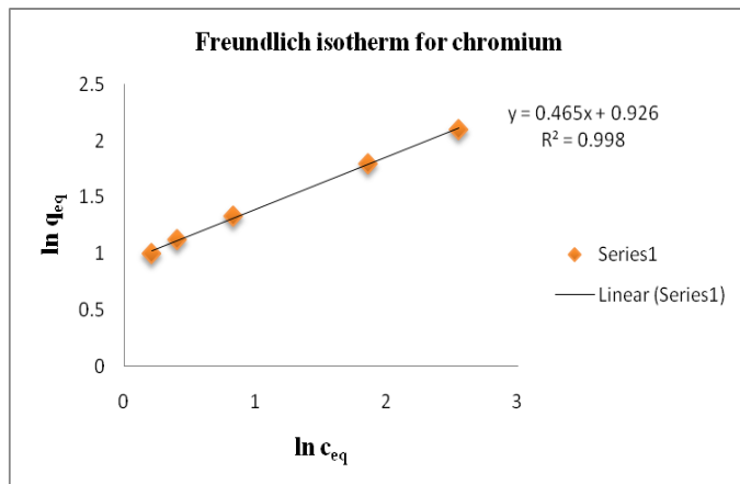
Fig 13: Freundlich isotherm plots for Chromium adsorption by activated Na-bentonite
