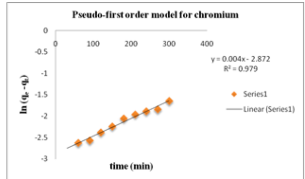
Fig 14: Pseudo first-order model for adsorption of chromium by activated Na-bentonite
