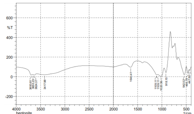
Fig 6: Interferogram of NA-bentonite
