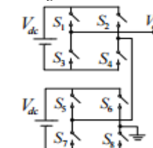
Fig 3: Cascaded H-bridge multilevel inverter
