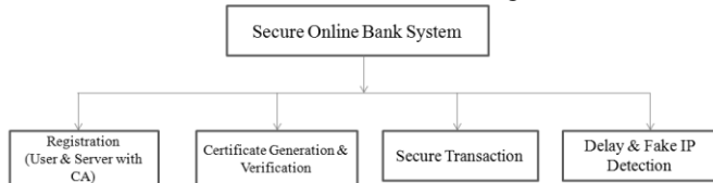
Fig 1 Structure chart
