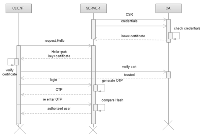
Fig 2. Sequence diagram
