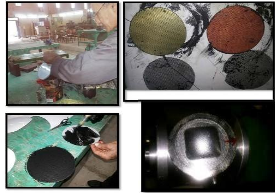
Figure 7 Specimen before and after deformation showing the preparation of painting the grid pattern of circles with special metal paint and after the deformation the new axes of these circles can be measured by a digital camera and programed software prepared for this work [5] to obtain the minor and major strain in order to get the forming limit diagram (F.L.D) and the forming limit curve (F.L.C) which they are a good representation of the formability of the sheet metal see Fig.8, 9.
