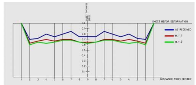
Figure 15 Thickness distribution profile of specimen made of 1060AA 1.00 mm thick (cross section B-B)
