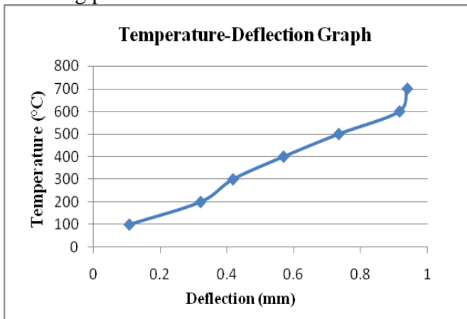
Temperature-deflection graph of ISWB 150
