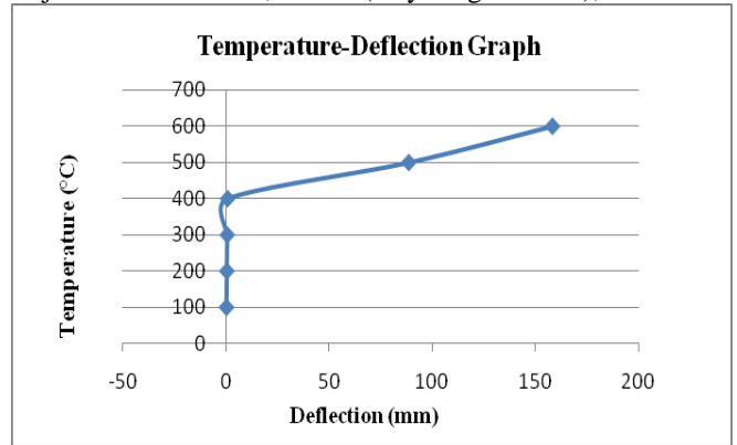
Temperature-deflection graph of ISWB 175
