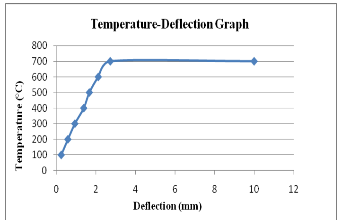
Temperature-deflection graph of ISWB 350
