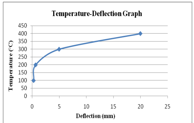
Temperature-deflection graph of ISWB 400
