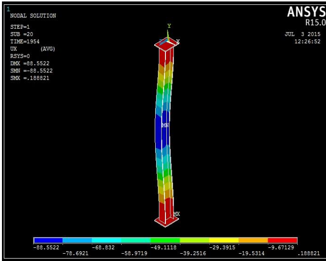
Buckling pattern of ISWB 175
