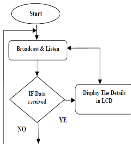
Fig. 3. Flow Chart of Bus Stop Module
