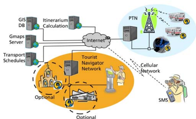
Fig.6. Architecture of the navigator service for a public transport network (PTN).
