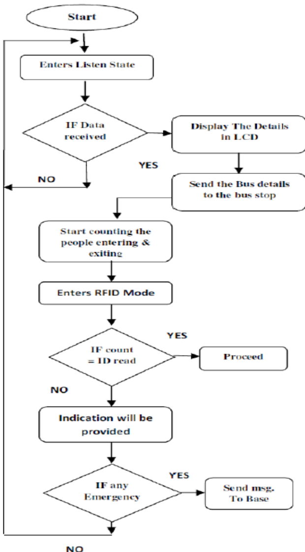
Fig. 4. Flow Chart of In Bus Module.
