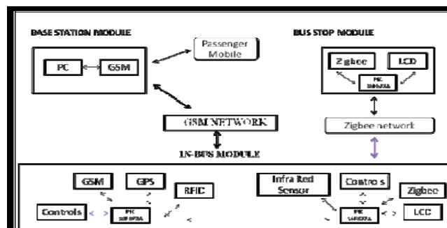
Fig. 2. Block diagram of THREE modules.
